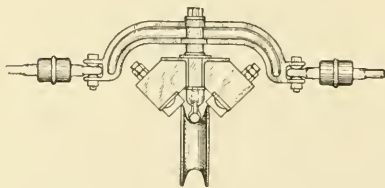
Fig. 220. Section of Block Switch
